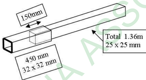
GALLOWS EXTENSION
